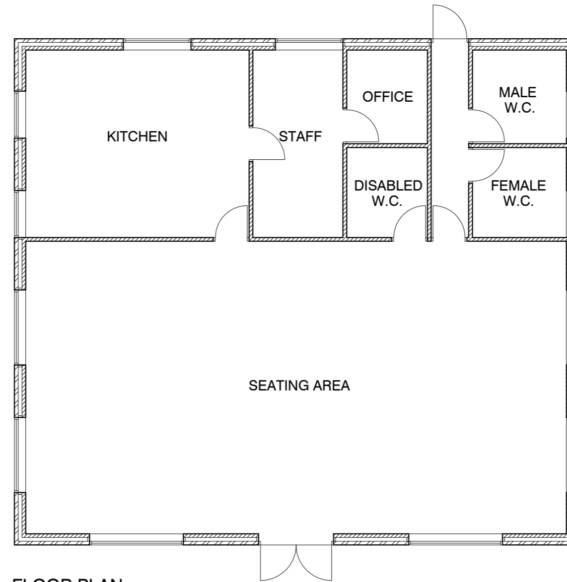
FLOOR PLAN
